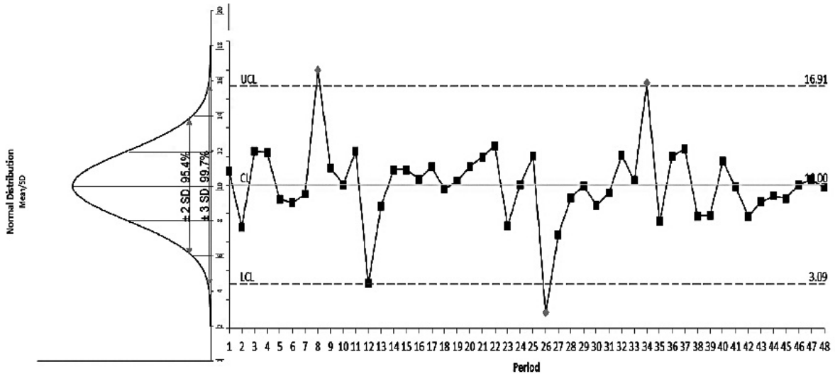
Figure 2.8 Control Chart and Probability theory 38
