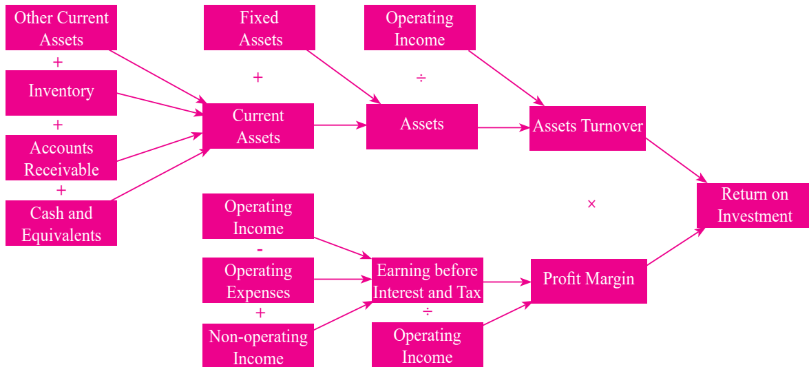
Figure 8.2 DuPont Model
